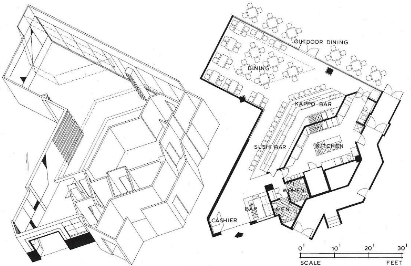
FLOOR PLAN
